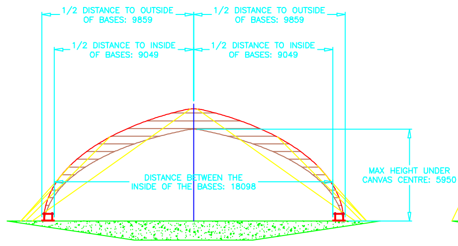
END VIEW ESTIMATED STAY POSITIONS INDICATED
