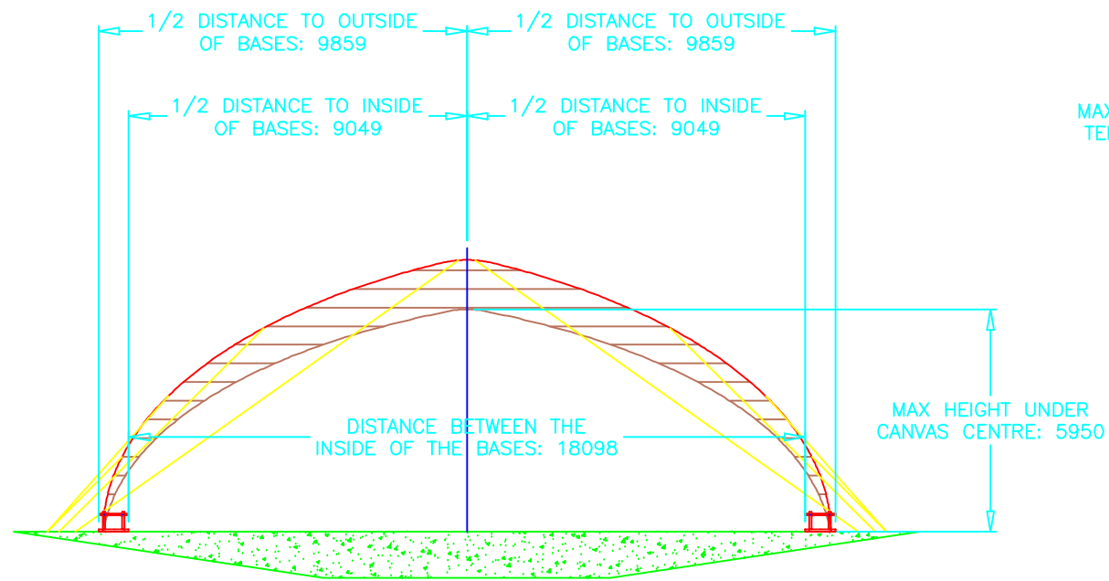
END VIEW ESTIMATED STAY POSITIONS INDICATED
